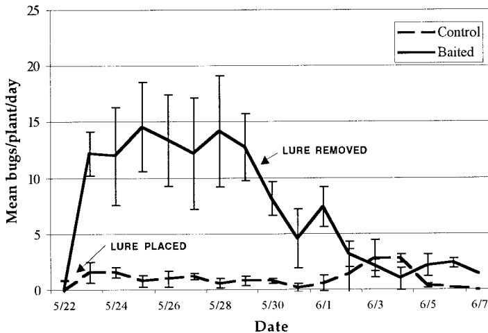
Fig. 2. Mean numbers of E. conspersus ( \pm SE) attracted to pheromone-baited (methyl 2E,4Z-decadienoate) or unbaited mullein showing bugs/plant. All plants had all stink bugs removed at outset, with lures removed from baited plants after 7 d, as indicated, n = 10 .
